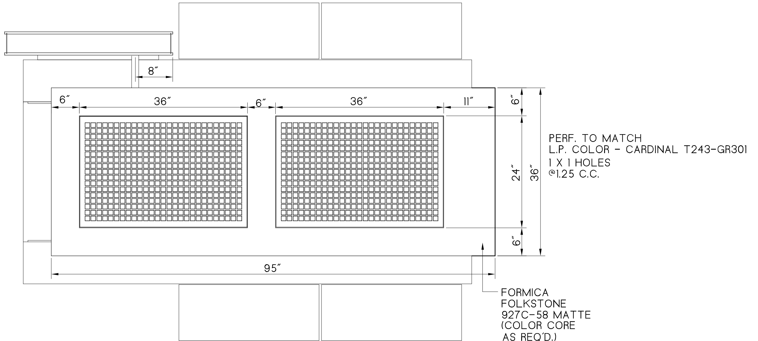
R O O F P L A N MIRACLE MILE RMU Sand Mountain, Inc. - 1/2/07
