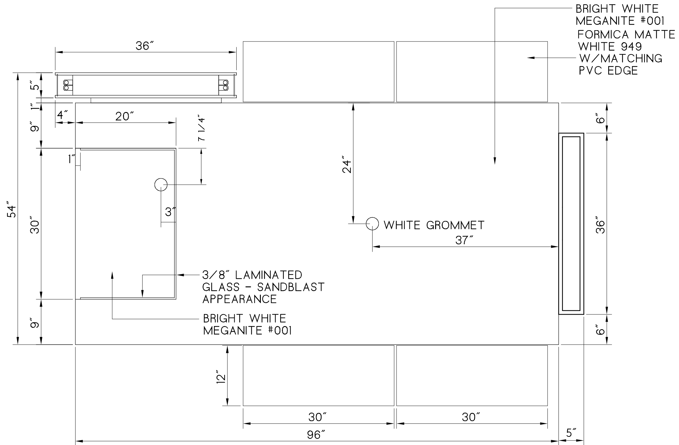
C O U N T E R P L A N MIRACLE MILE RMU Sand Mountain, Inc. - 1/2/07
