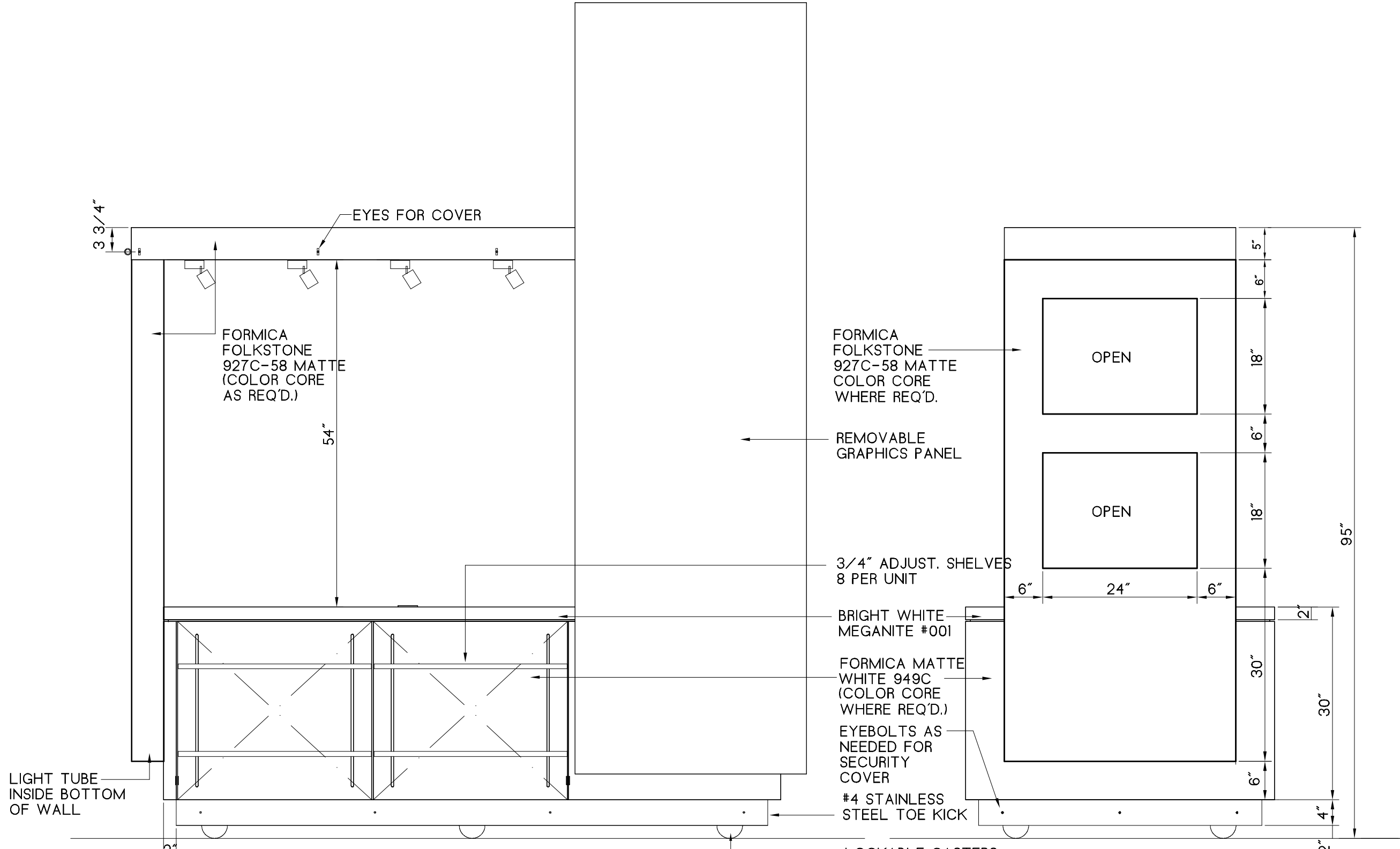
TOWER SIDE ELEVATION MIRACLE MILE RMU Sand Mountain, Inc. - 1/2/07
